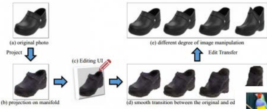
Fig. 1. We use generative adversarial networks (GAN) [12] to perform on the natural image manifold. We first project an original photo I to a low-dimensional latent vector z_0 . We then use an interactive image editing UI to modify the color and shape of the object (for example, dragging the object to change its geometric and color change). This process is controlled by our interactive image editing UI.
