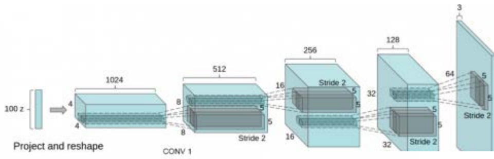
Figure 1: DCGAN generator used for LSUN scene motion Z is projected to a small spatial extent convolution. A series of four fractionally-strided convolutions (in series) and deconvolutions (in series) then convert this high level representation into a fully connected or pooling layers are used.
